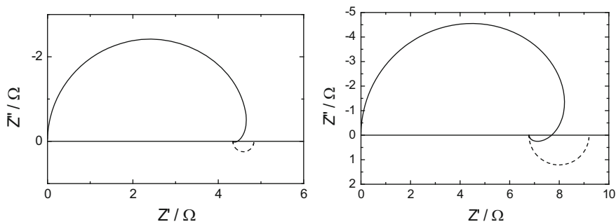
Fig. 5.4 Complex plane plots of faradaic ( dashed lines ) and total ( continuous lines ) impedances where B > 0, C_{dl} = 25 \mu\text{F} ; left : \eta = -0.095 \text{ V}, \beta_1 = \beta_2 = 0.5, k_1 = 10^{-6.65}, k_{-1} = 10^{-9.2}, k_2 = 10^{-8.05} \text{ mol cm}^{-2} \text{ s}^{-1}, R_{ct} = 4.835 \Omega, R_0 = 42.76 \Omega, L = 0.0471 \text{ H} ; right : \eta = -0.14 \text{ V}, \beta_1 = 0.7, \beta_2 = 0.3, k_1 = 10^{-9.2}, k_{-1} = 10^{-8.05}, k_2 = 10^{-6.35} \text{ mol cm}^{-2} \text{ s}^{-1}, R_{ct} = 9.2 \Omega, R_0 = 25.7 \Omega, L = 0.0241 \text{ H}
