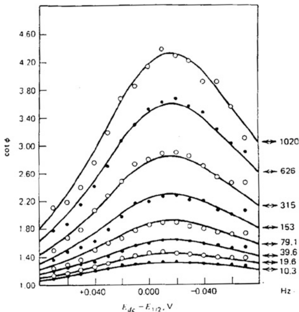
Fig. 4.9 Dependence of \cot \phi on potential for reduction of \text{TiCl}_4 in solution containing \text{H}_2\text{C}_2\text{O}_4 measured at different frequencies (Reprinted with permission from Ref. [153]. Copyright 1963 American Chemical Society)
